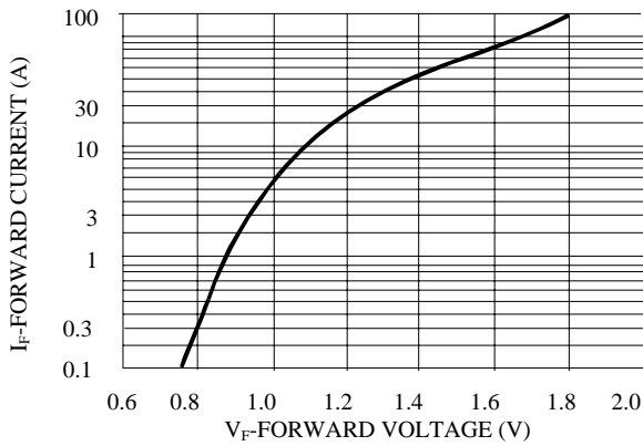
Fig. 5-TYPICAL FORWARD CHARACTERISTICS
